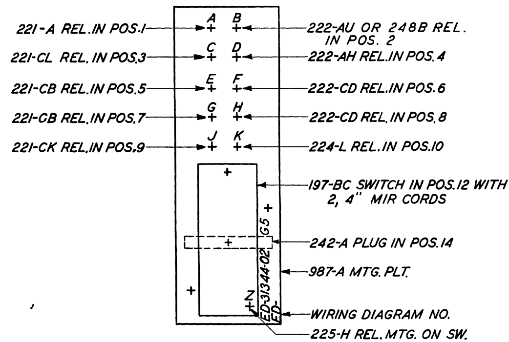
MOUNTING PLATE EQUIPMENT FIG. 1
